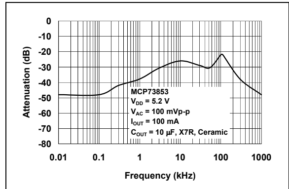
FIGURE 2-18: Power Supply Ripple Rejection.
