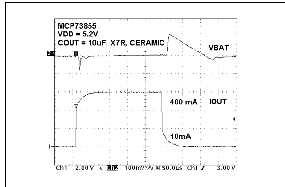
FIGURE 2-17: Load Transient Response.
