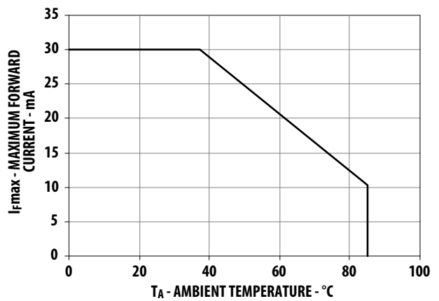
Figure 9 Maximum Forward Current vs. Ambient Temperature
