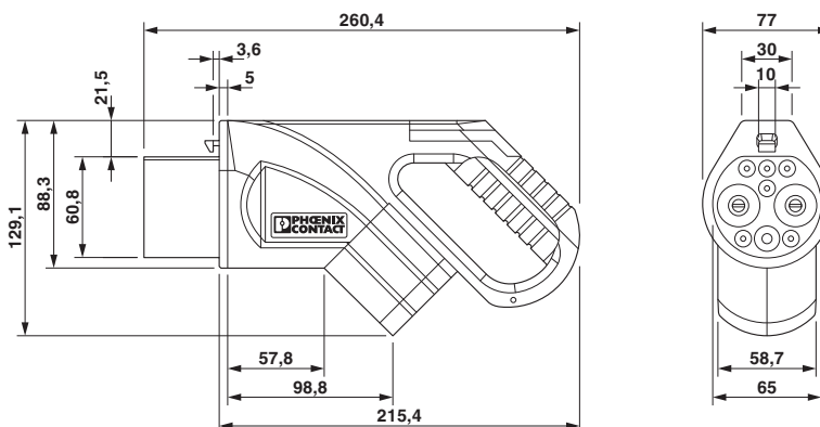
Dimensional drawing
