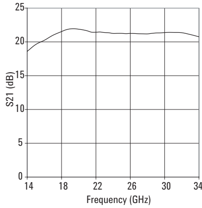
Figure 1. Typical Gain
