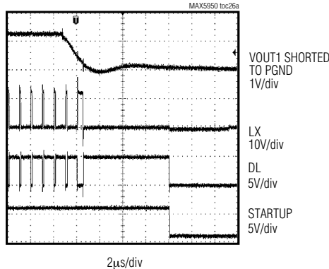
SHORT-CIRCUIT RESPONSE
