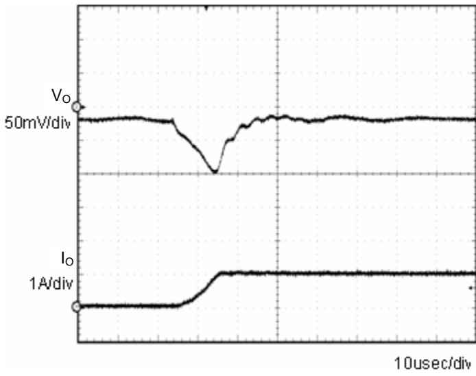
Fig.2 Transient Response (0→1.0A) Co=1μF
