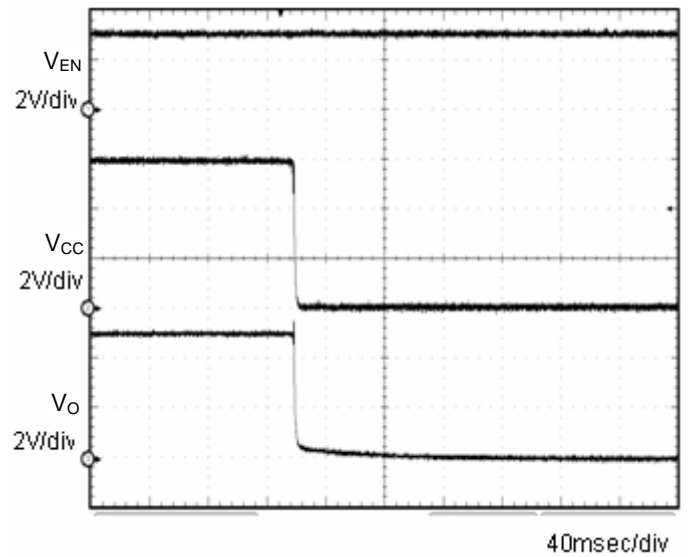
Fig.5 OFF sequence 1 Co=1μF
