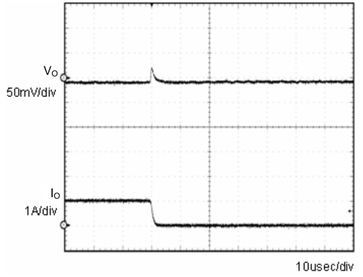
Fig.3 Transient Response (1.0→0A) Co=1μF
