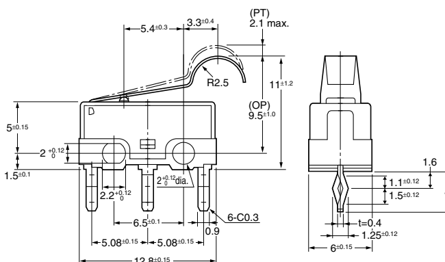
External dimensions
