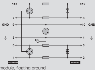
Complete module, floating ground
