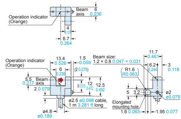
PM-R25 Sensor
