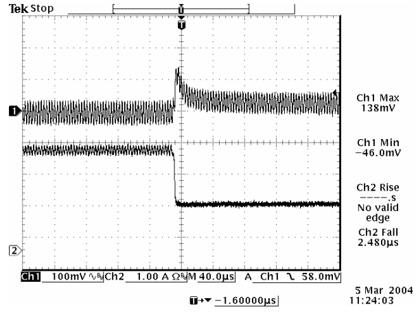
100% to 50% load Transient at Vin=5 V, Vo= 2.5 V
