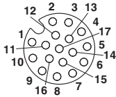
Pin assignment M12, 12-pos., female side view
