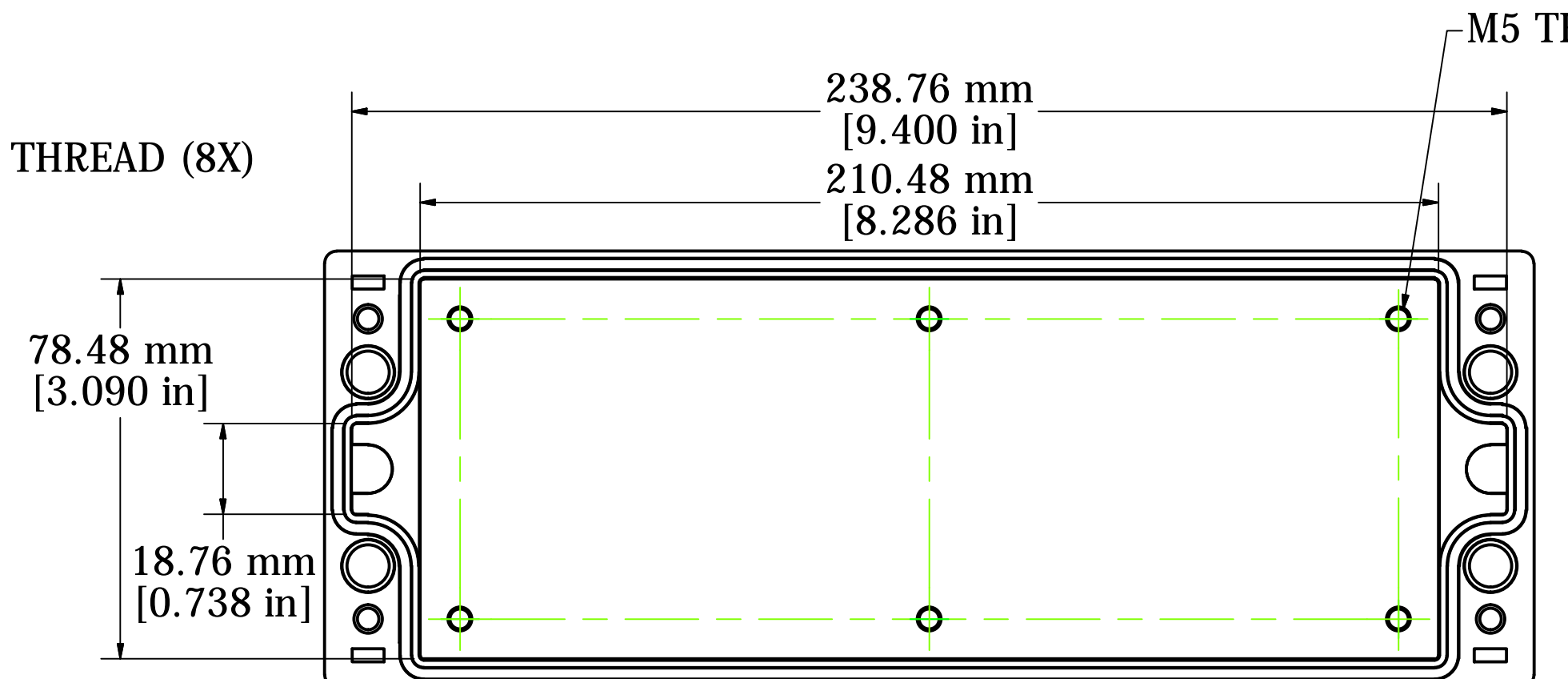
LID - INSIDE VIEW
