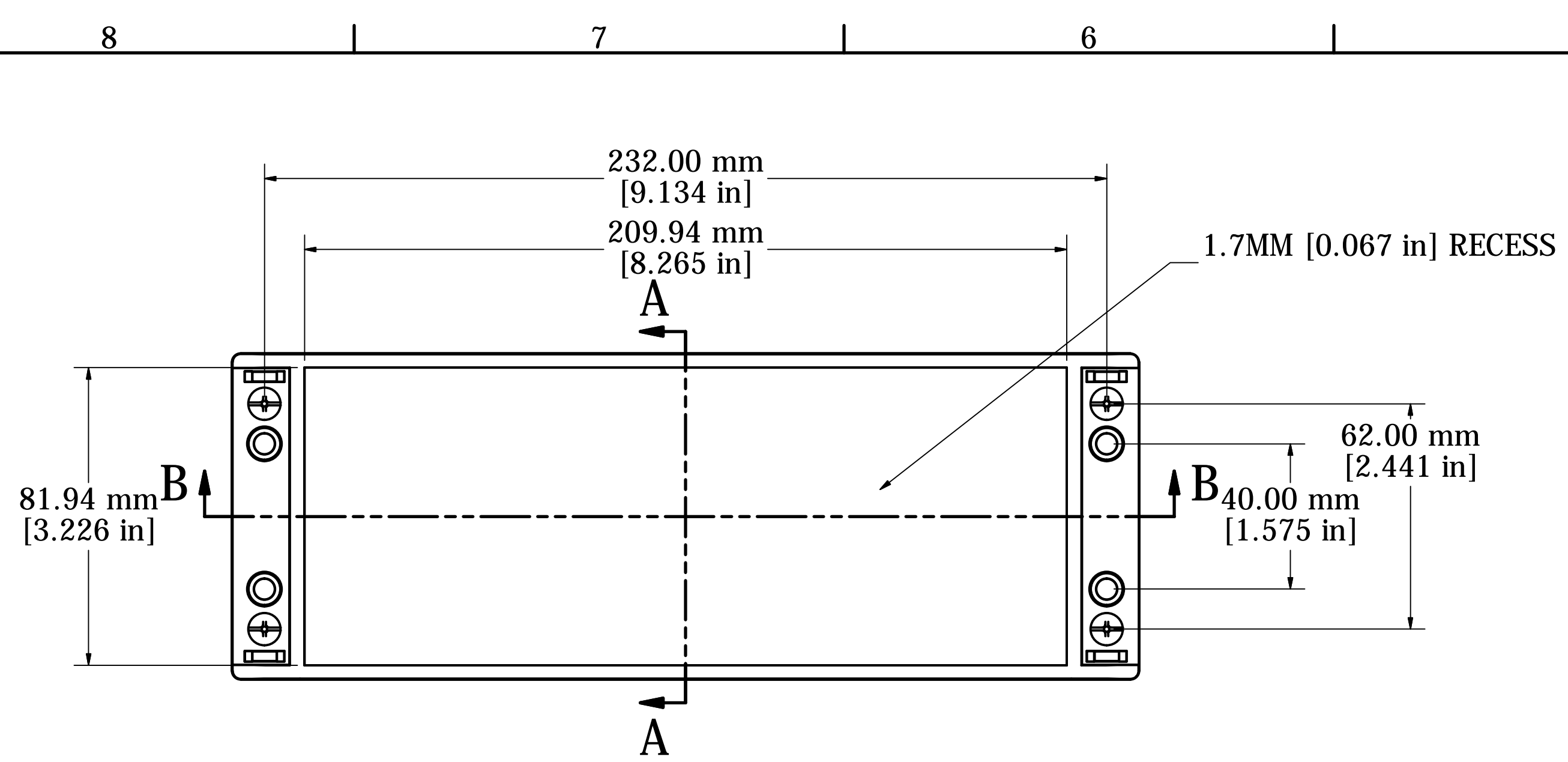
ASSEMBLY - TOP VIEW
