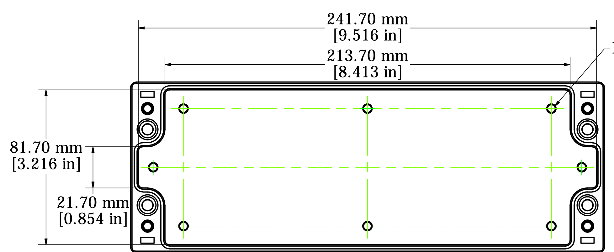
BOX - INSIDE VIEW
