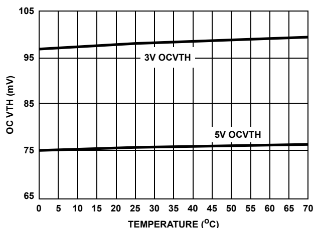
FIGURE 2. OC VTH vs TEMPERATURE ( V_{R_{OCSET}} = 1.21V )
