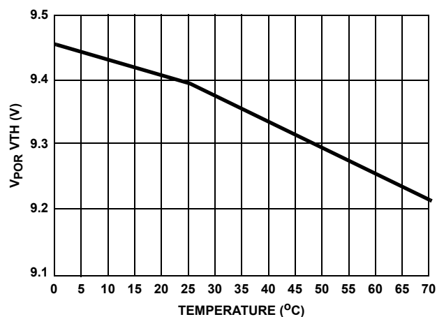
FIGURE 4. V_{CC} POWER ON RESET VTH vs TEMPERATURE
