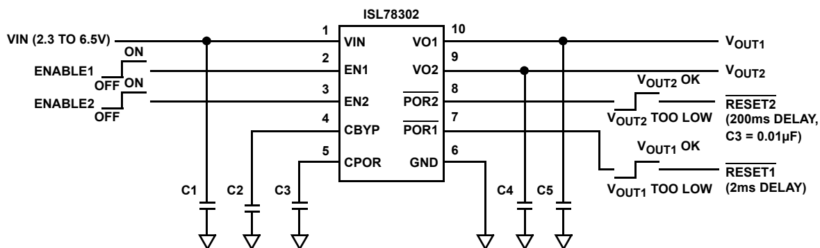
C1, C4, C5: 1μF X5R CERAMIC CAPACITOR C2: 0.01μF X7R CERAMIC CAPACITOR C3: 0.01μF X7R CERAMIC CAPACITOR
