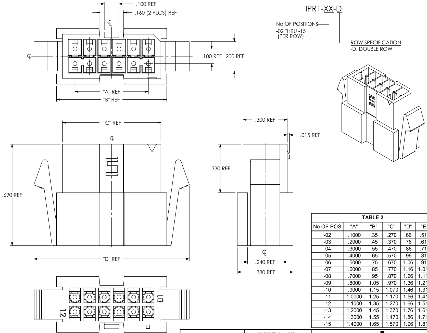
FIG 1 IPR1-06-D SHOWN
