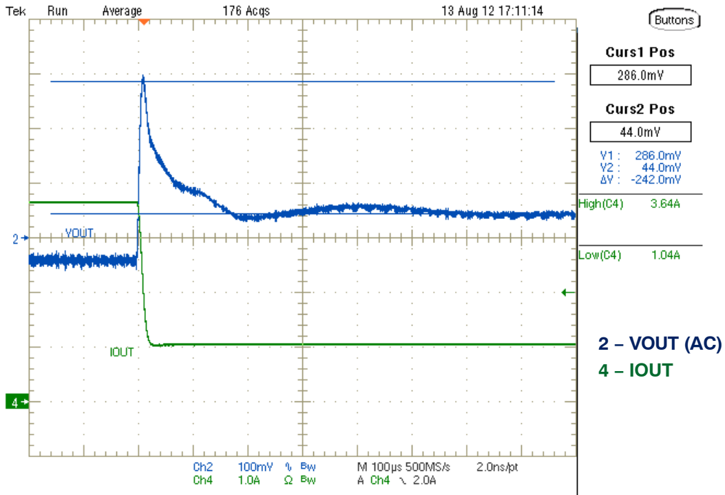
Figure 24. V_{IN} = 230 V_{AC} , I_{OUT} = 3.5 - 1.0 A , V_{OUT\_OVERSHOOT} = 242 mV
