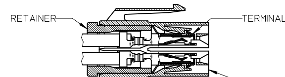
TERMINAL AND RETAINER ASSEMBLY DRAWING
