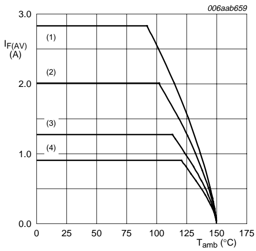
Ceramic PCB, Al_2O_3 , standard footprint T_j = 150\text{ }^\circ\text{C} (1) \delta = 1 ; DC (2) \delta = 0.5 ; f = 20\text{ kHz} (3) \delta = 0.2 ; f = 20\text{ kHz} (4) \delta = 0.1 ; f = 20\text{ kHz}
