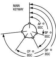
PLUG (front face shown)
