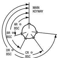
RECEPTACLE (front face shown)
