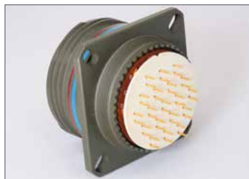
D38999 Connector with PC Tail Coax Contacts, Sealing Plugs in unused contact cavities and PC Tail Alignment Disc
