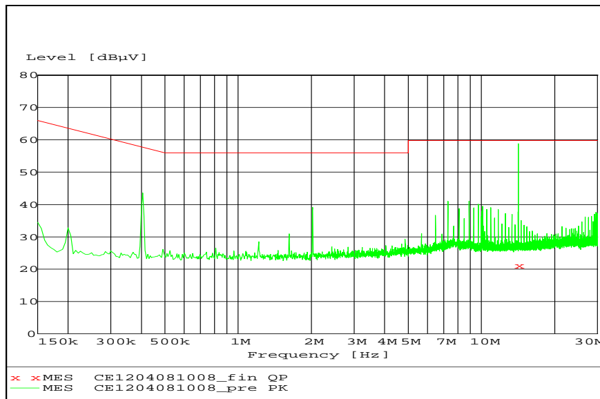
Figure 25. EMC Considerations
