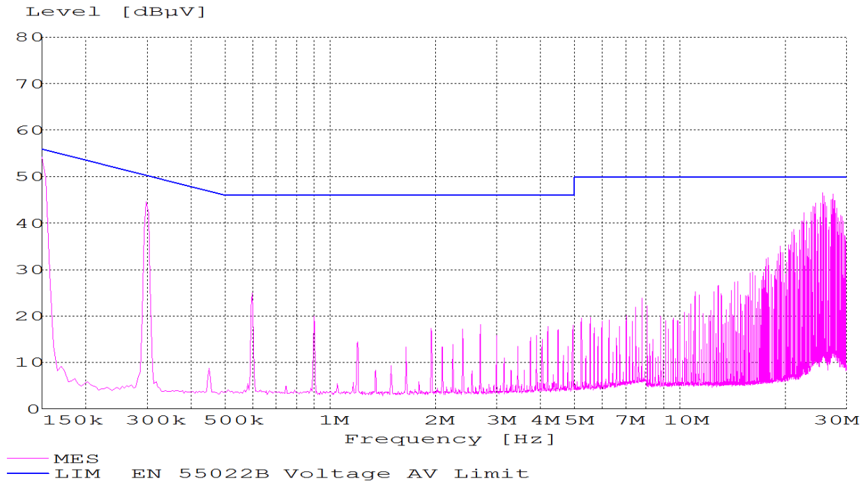
Figure 25. EMC Considerations
