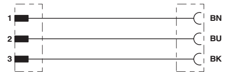
Contact assignment of the DEUTSCH connectors
