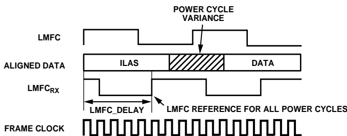
Figure 102. LMFC_DELAY_x to Compensate for Link Delay > LMFC
