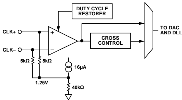
Figure 131. Clock Input
