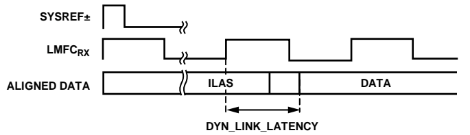
Figure 104. DYN_LINK_LATENCY_x Illustration
