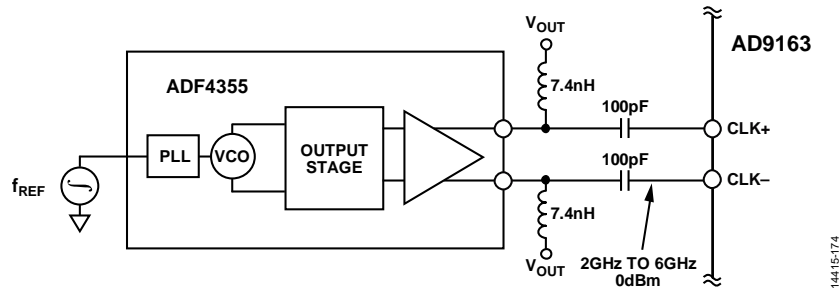
Figure 133. Possible Signal Chain for CLK± Input
