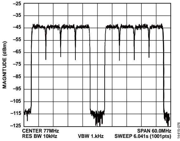
Figure 83. Gap Channel ACLR at 77 MHz
