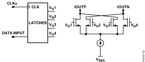
Figure 126. Quad-Switch Architecture
