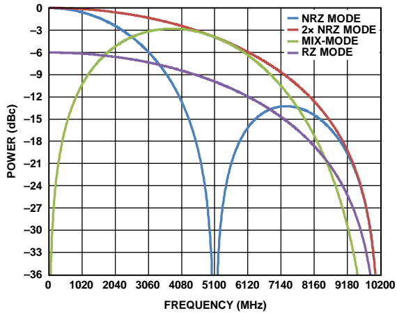
Figure 130. Sinc Roll-Off with 2x NRZ Mode Added, f_{DAC} = 5.1 GSPS
