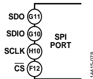
Figure 85. Serial Port Interface Pins
