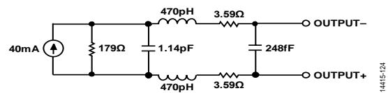
Figure 139. Equivalent Circuit Model of the DAC Output
