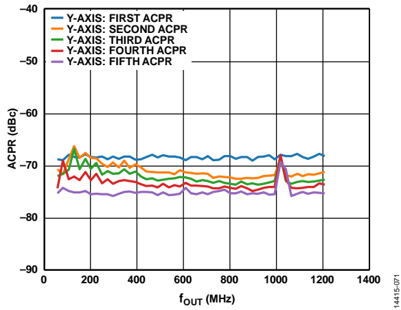
Figure 78. Four-Carrier ACPR vs. f_{OUT}
