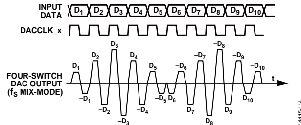
Figure 128. Mix-Mode Waveform
