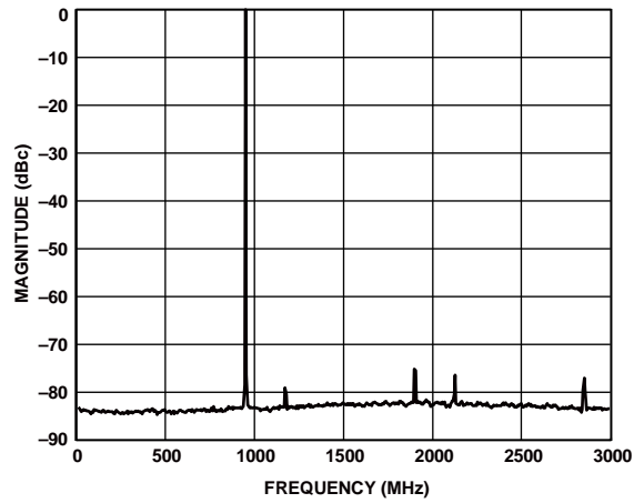
Figure 68. Single Carrier at 950 MHz Output (Shuffle On)
