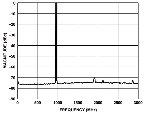
Figure 69. Four Carriers at 950 MHz Output (Shuffle On)
