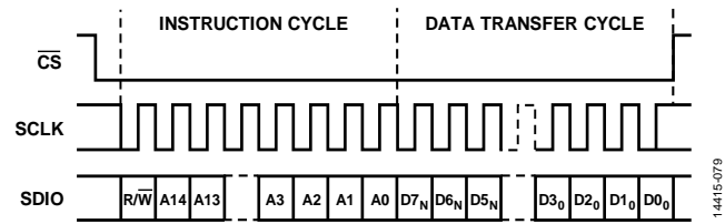
Figure 86. Serial Register Interface Timing, MSB First, Register 0x000, Bit 5 and Bit 2 = 0
