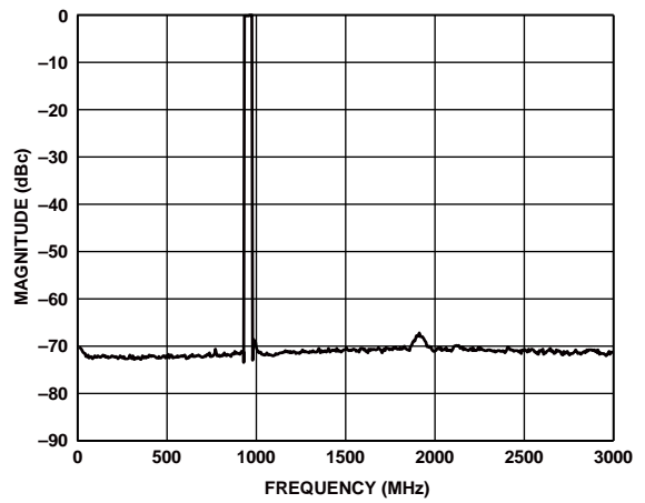
Figure 70. Eight Carriers at 950 MHz Output (Shuffle On)
