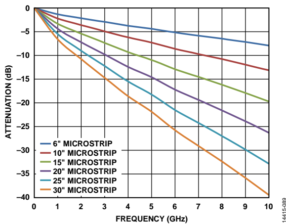
Figure 96. Insertion Loss of 50 Ohm Microstrips on FR4
