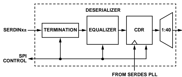
Figure 91. Deserializer Block Diagram
