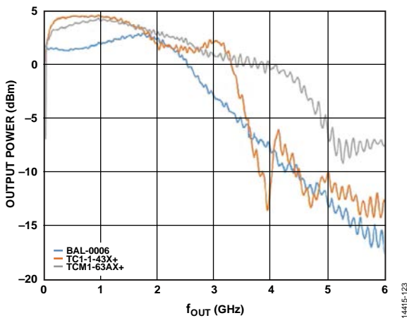
Figure 137. Measured DAC Output Response; f DAC = 6 GSPS
