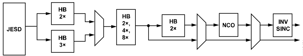
Figure 107. Block Diagram of the Main Digital Datapath
