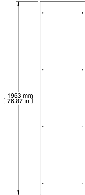
FRONT VIEW
