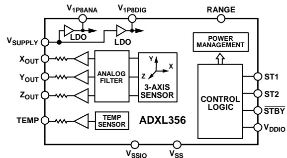
Figure 1. ADXL356
