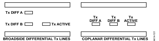
Figure 125. Broadside vs. Coplanar Differential Stripline Routing Techniques
