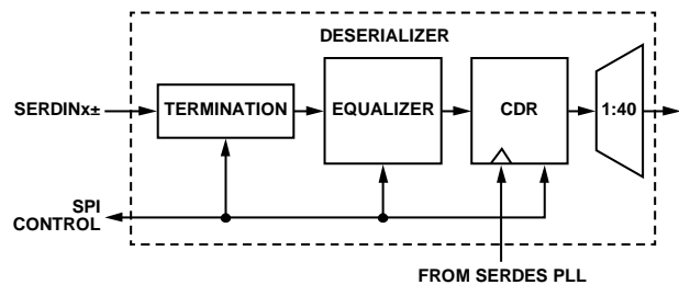
Figure 92. Deserializer Block Diagram
