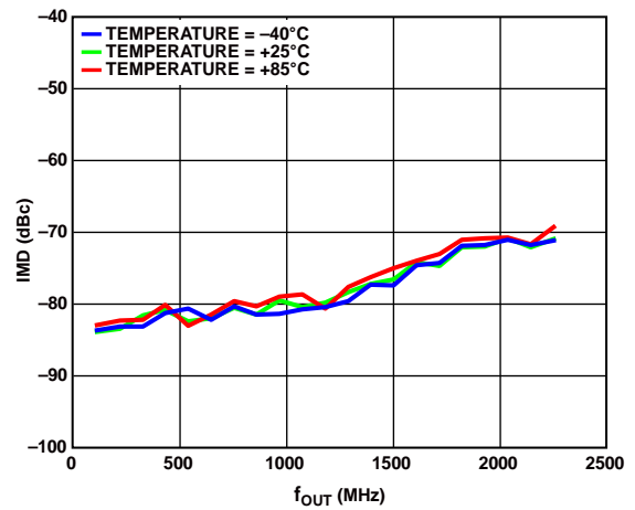
Figure 29. IMD vs. f_{OUT} over Temperature
