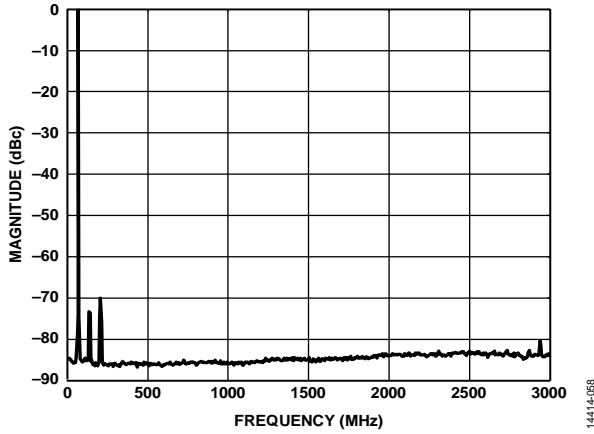
Figure 60. Single Carrier at 70 MHz Output
