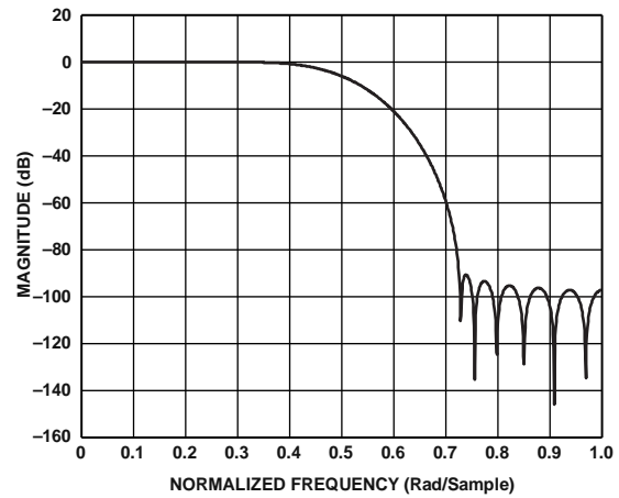
Figure 116. Second 2x Half-Band 45% Filter Response
