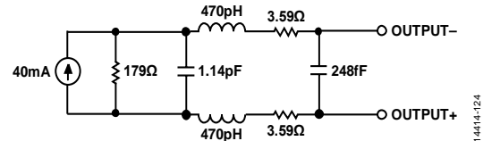
Figure 141. Equivalent Circuit Model of the DAC Output
