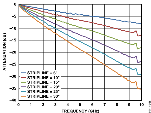
Figure 96. Insertion Loss of 50 Ohm Striplines on FR4
