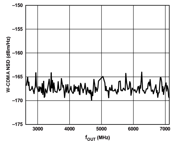
Figure 47. W-CDMA NSD vs. f_{OUT}
