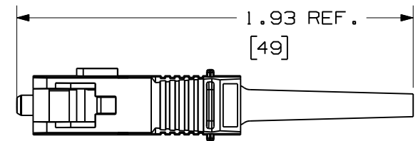
SC CONNECTOR WITH 900um BOOT (SHOWN WITHOUT DUST CAP)
