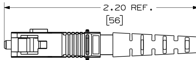
SC CONNECTOR WITH 3mm BOOT (SHOWN WITHOUT DUST CAP)
