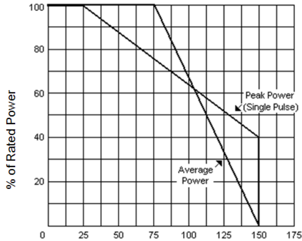
FIGURE 2 Lead Length = 3/8"
