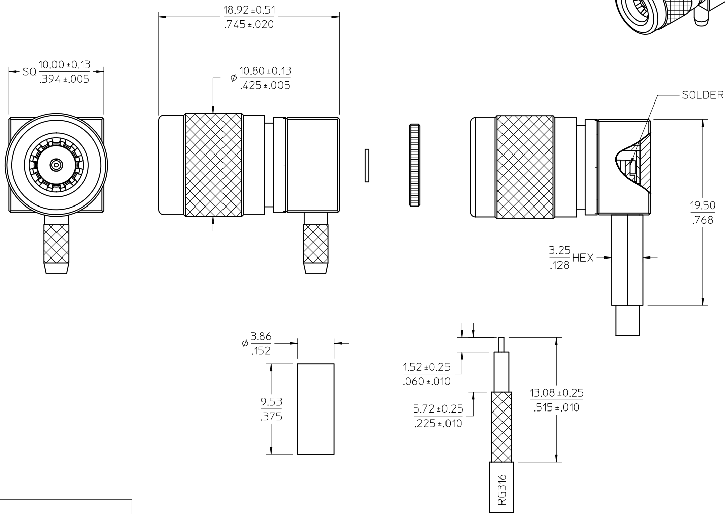
STRIPPING DIMENSIONS
