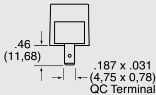
4 – Quick Connect .187"
