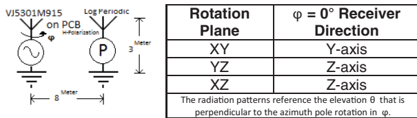
Fig. 3 - VJ5301M915 PCB Mounting and Coordinate Directions
