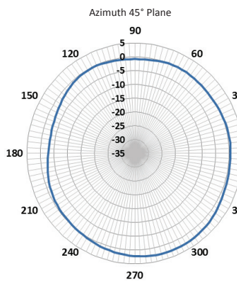
1690 MHz
