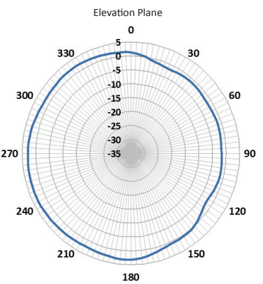
1690 MHz
